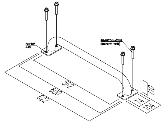
<図1>Pablo AS 寸法図
